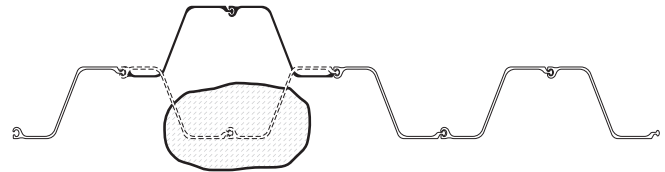
Layout to Avoid an Obstruction
